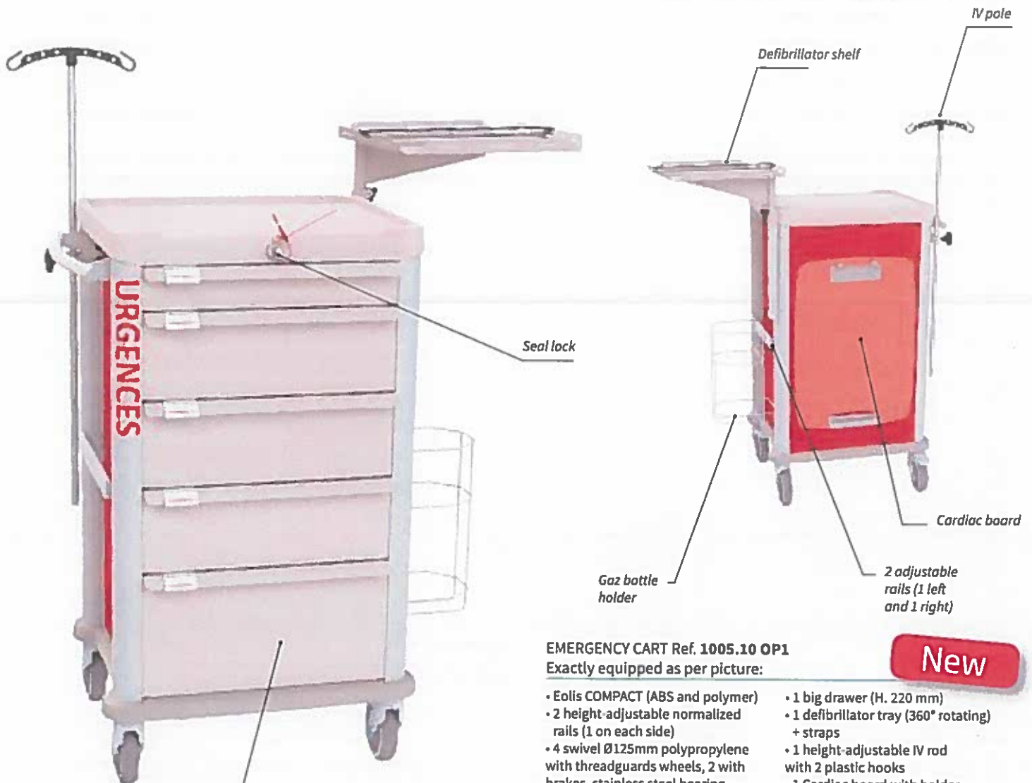
Epoxy steel drawers with integrated telescopic slides and label holders (label not included)
